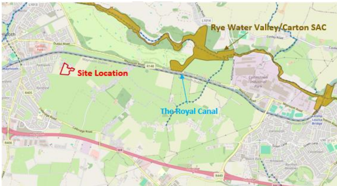
Figure 2 Flow network and hydrological links to the Rye Water Valley/Carton SAC (EPA, 2025)
